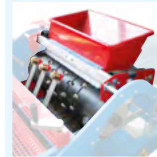
14 Drum for big seeds , as for ex. acorns.
